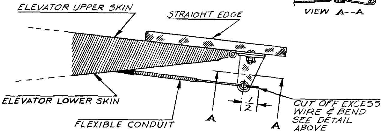
SKETCH 4 METHOD OF SETTING TRIM TAB
