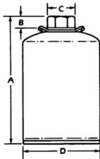
Popular spin-on oil filters
