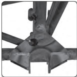
Float Fitting
